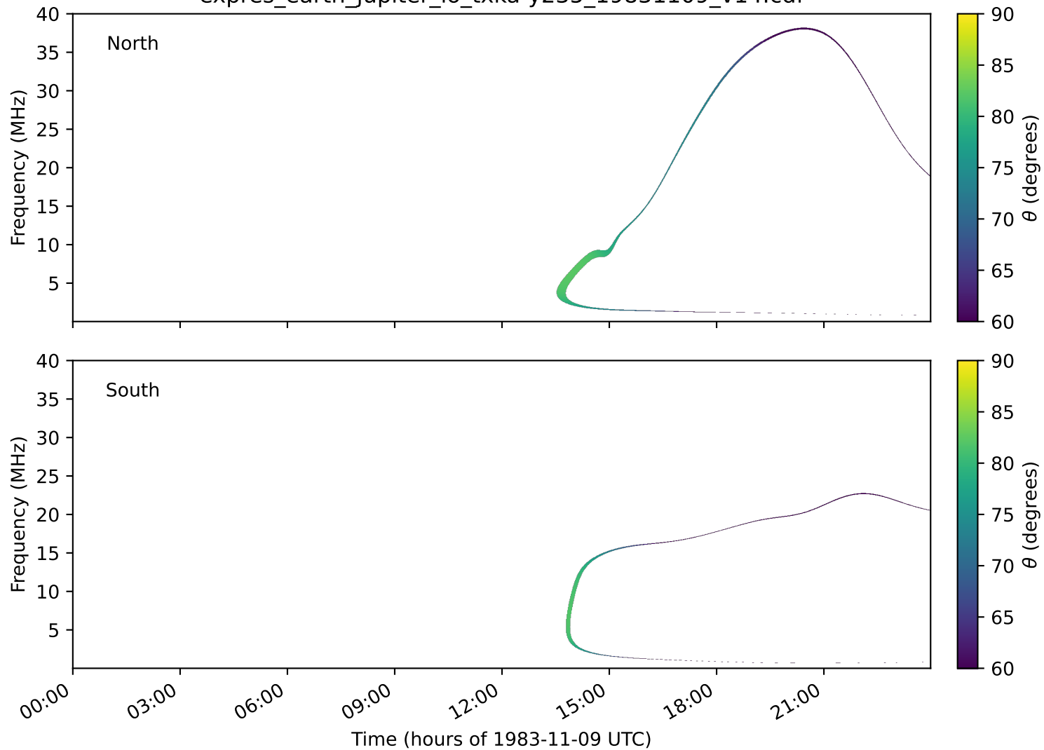
expres_earth_jupiter_io_txka-y235_19831109_v14.cdf
