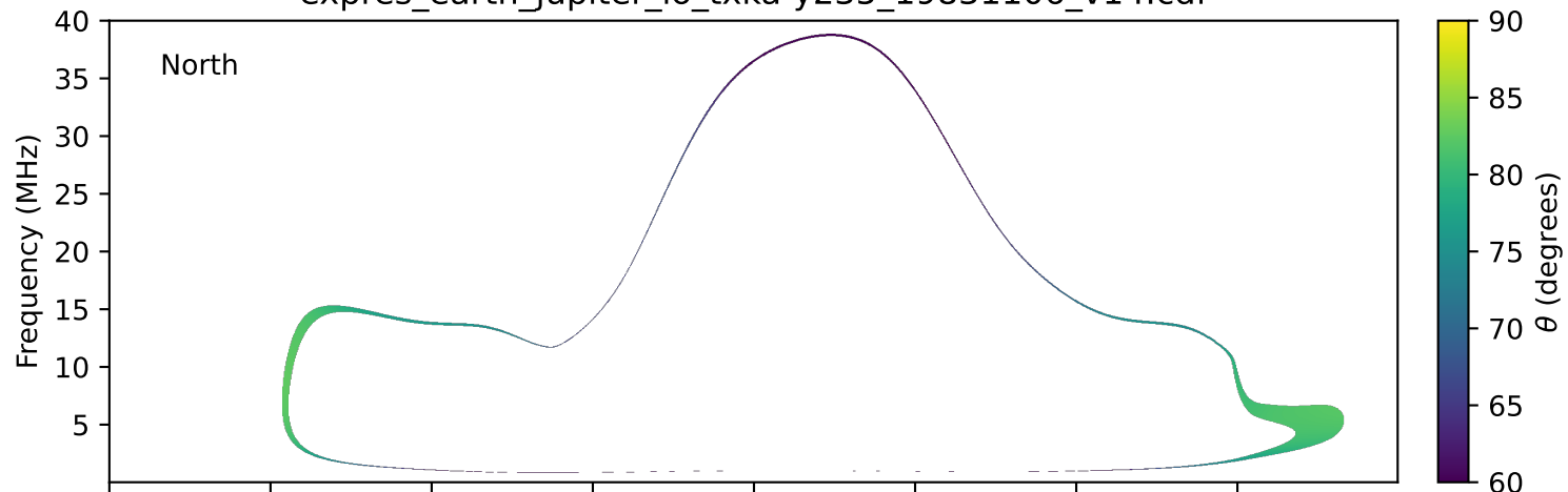
expres_earth_jupiter_io_txka-y235_19831106_v14.cdf
