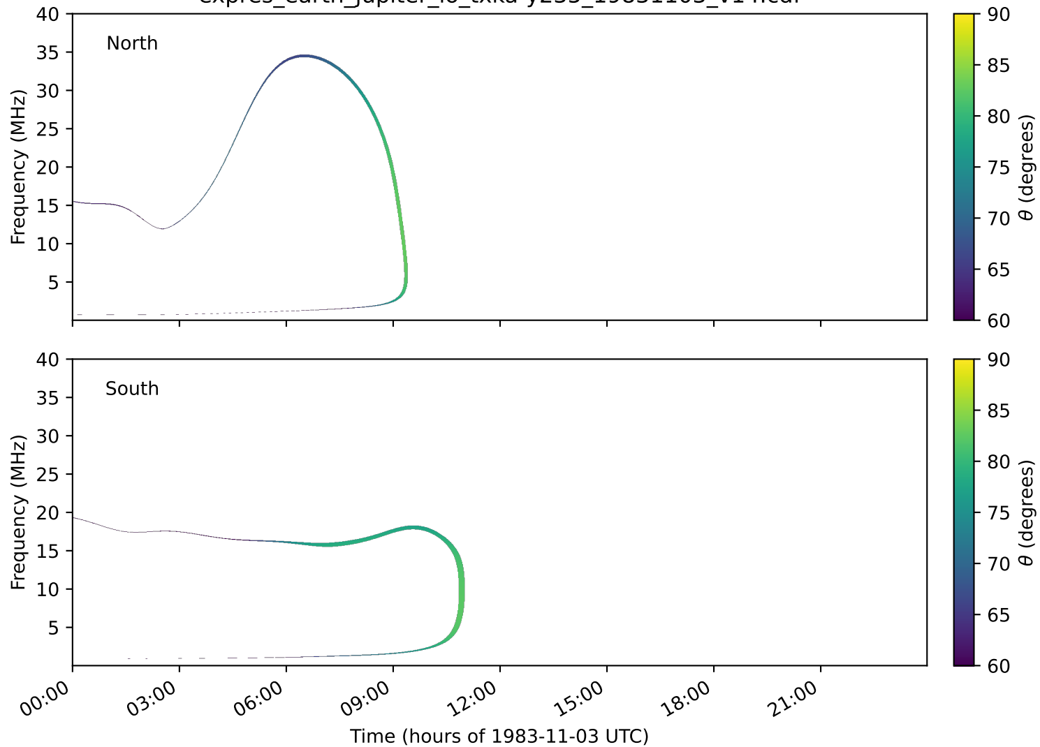
expres_earth_jupiter_io_txka-y235_19831103_v14.cdf
