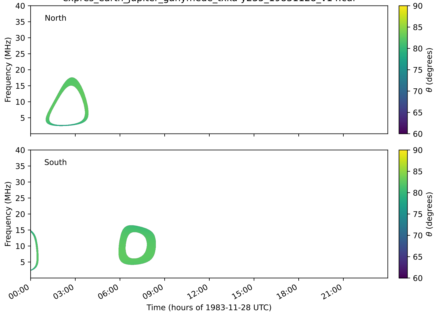
expres_earth_jupiter_ganymede_txka-y235_19831128_v14.cdf
