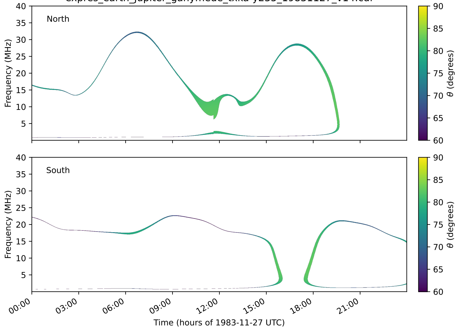
expres_earth_jupiter_ganymede_txka-y235_19831127_v14.cdf
