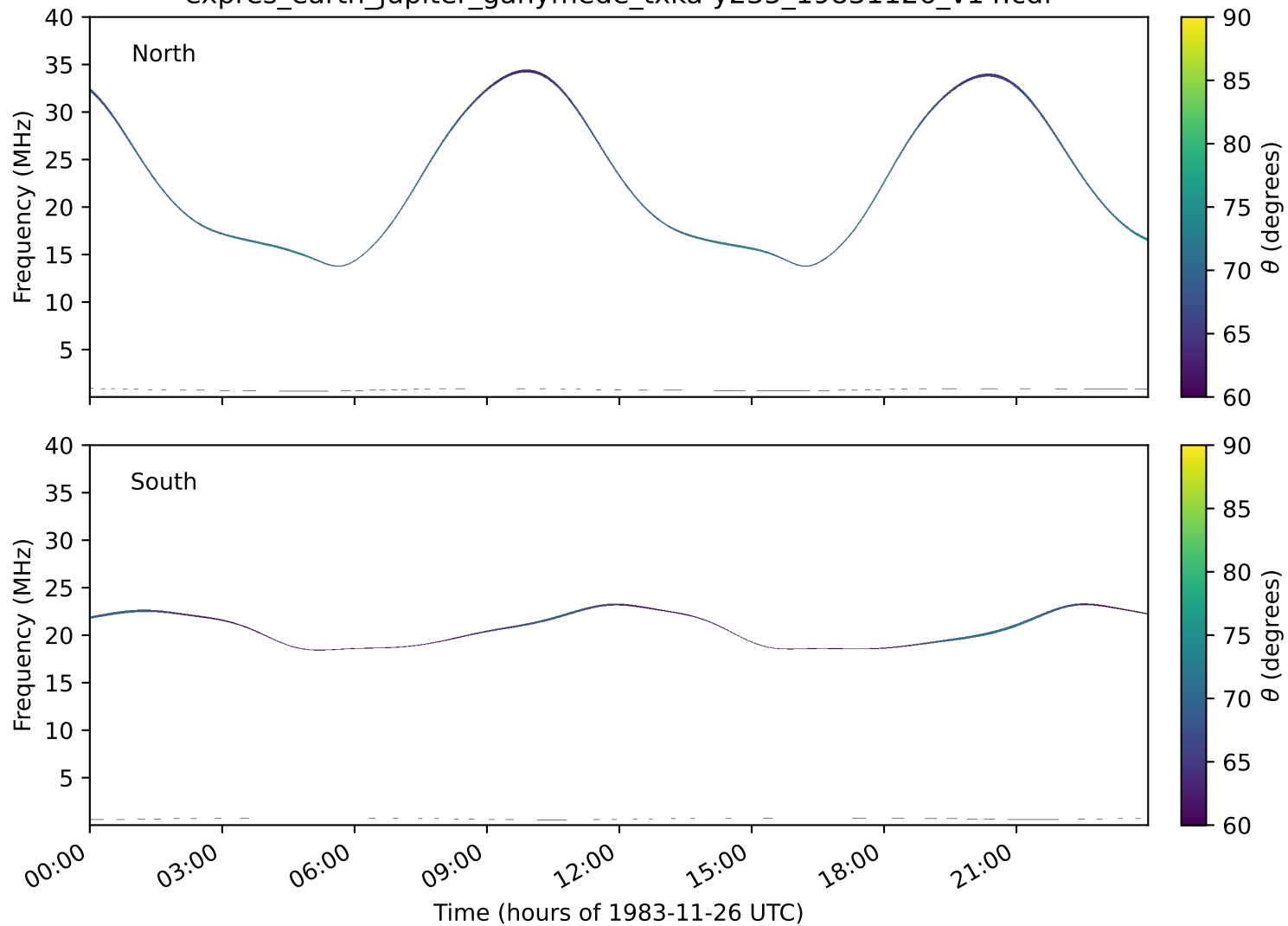
expres_earth_jupiter_ganymede_txka-y235_19831126_v14.cdf
