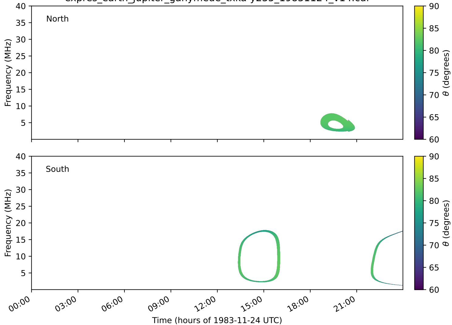
expres_earth_jupiter_ganymede_txka-y235_19831124_v14.cdf
