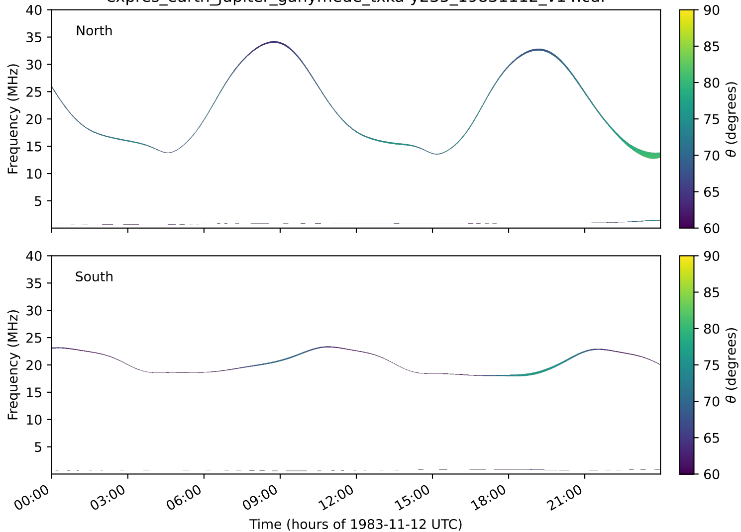
expres_earth_jupiter_ganymede_txka-y235_19831112_v14.cdf
