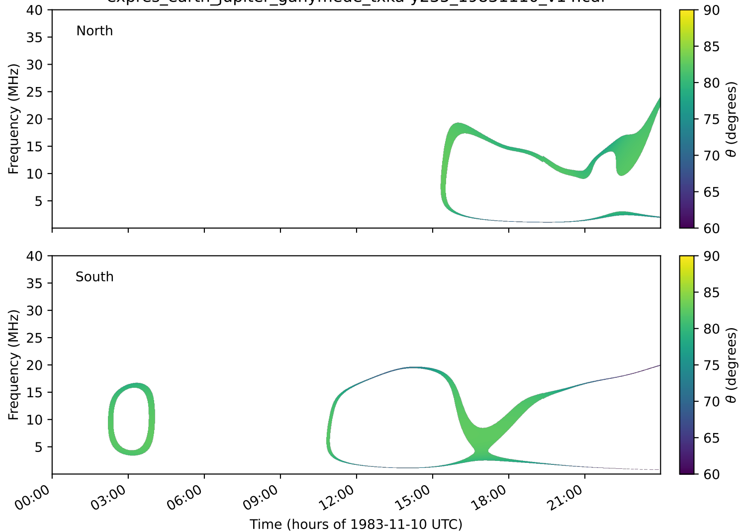
expres_earth_jupiter_ganymede_txka-y235_19831110_v14.cdf
