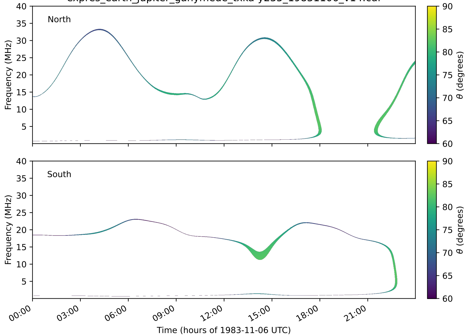
expres_earth_jupiter_ganymede_txka-y235_19831106_v14.cdf
