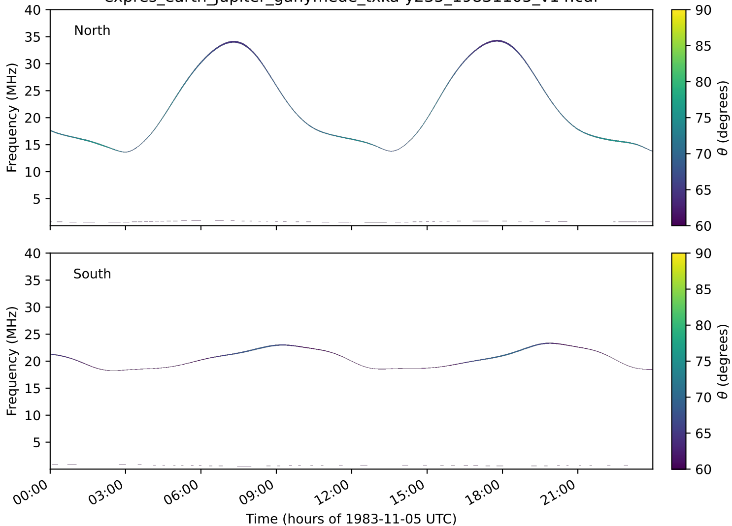
expres_earth_jupiter_ganymede_txka-y235_19831105_v14.cdf
