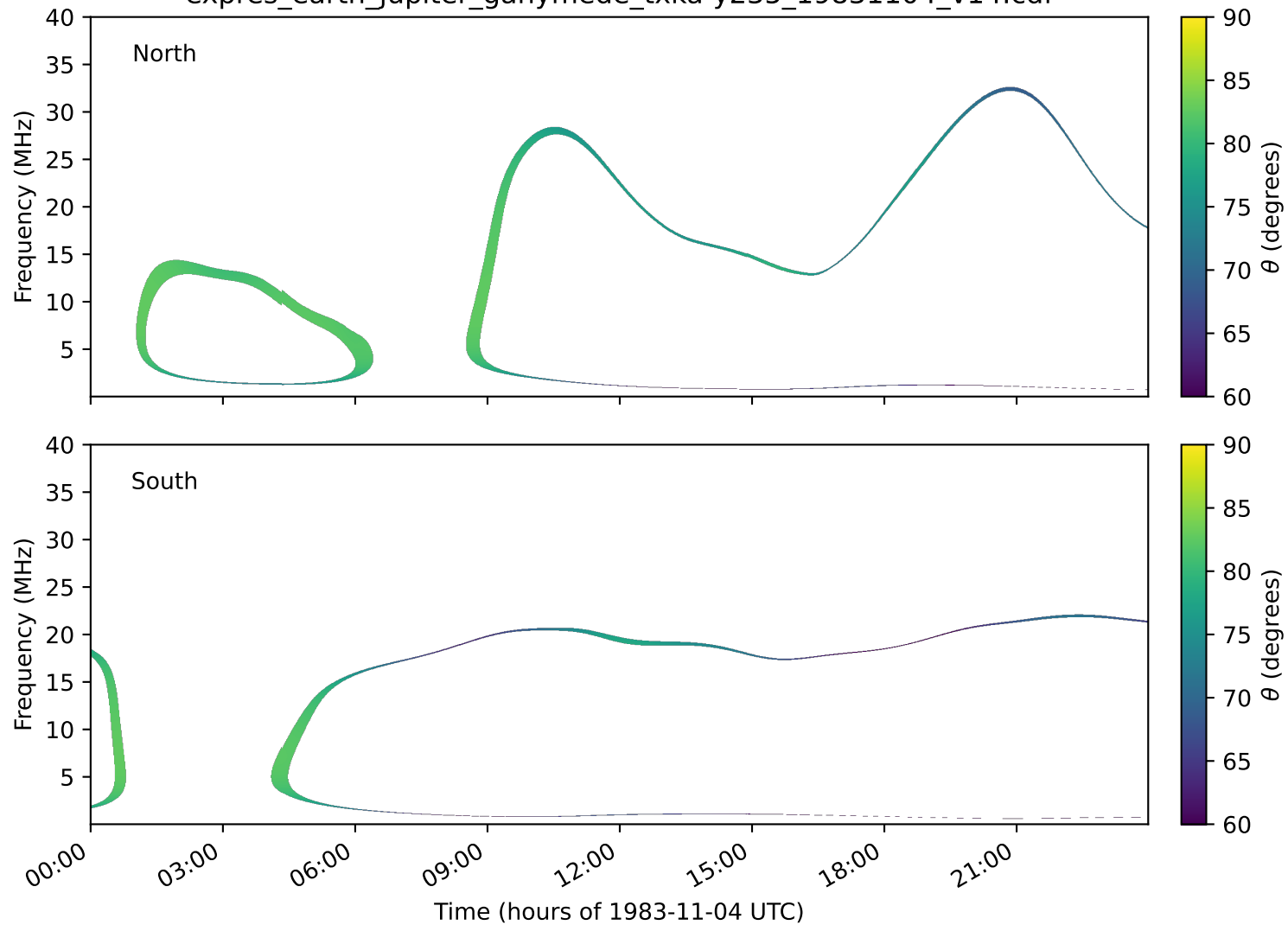
expres_earth_jupiter_ganymede_txka-y235_19831104_v14.cdf
