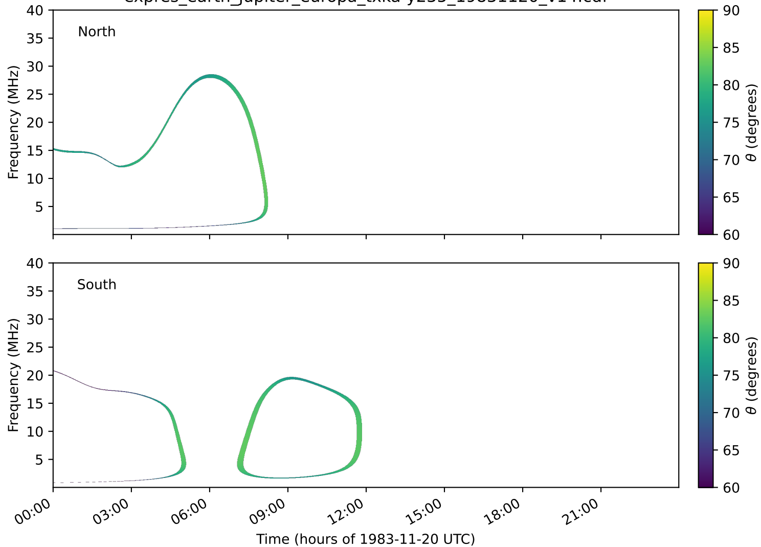
expres_earth_jupiter_europa_txka-y235_19831120_v14.cdf
