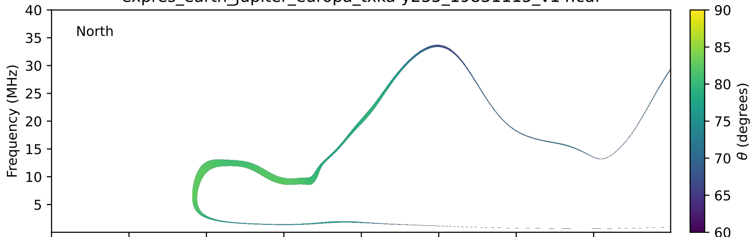
expres_earth_jupiter_europa_txka-y235_19831115_v14.cdf
