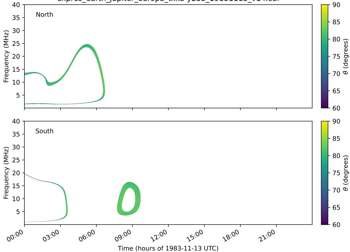
expres_earth_jupiter_europa_txka-y235_19831113_v14.cdf
