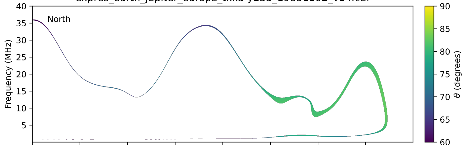
expres_earth_jupiter_europa_txka-y235_19831102_v14.cdf
