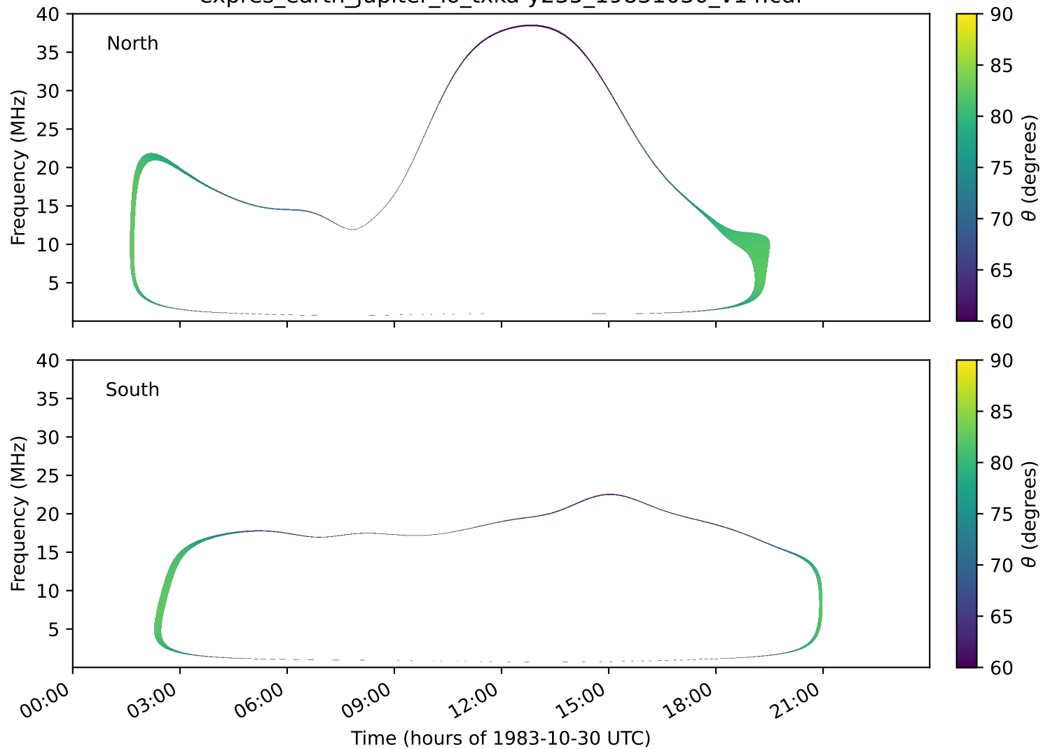
expres_earth_jupiter_io_txka-y235_19831030_v14.cdf
