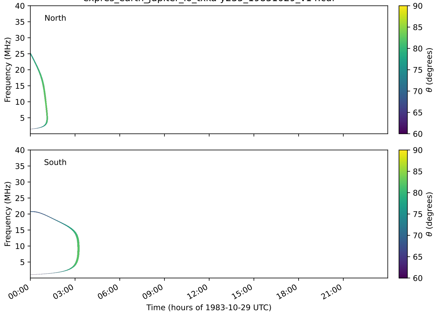
expres_earth_jupiter_io_txka-y235_19831029_v14.cdf
