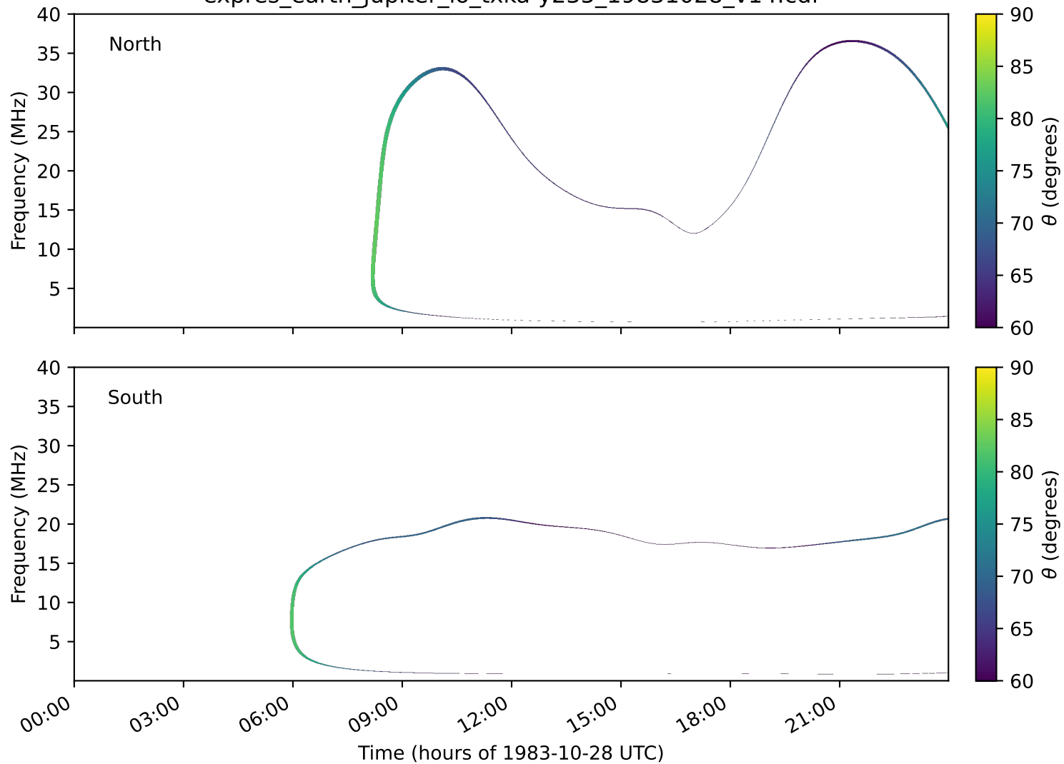
expres_earth_jupiter_io_txka-y235_19831028_v14.cdf
