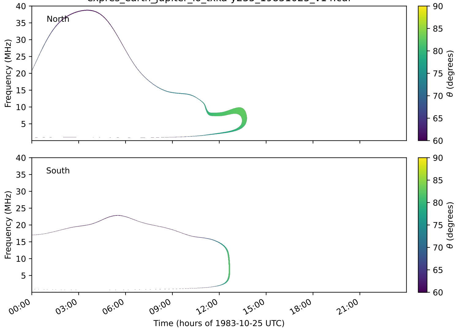
expres_earth_jupiter_io_txka-y235_19831025_v14.cdf
