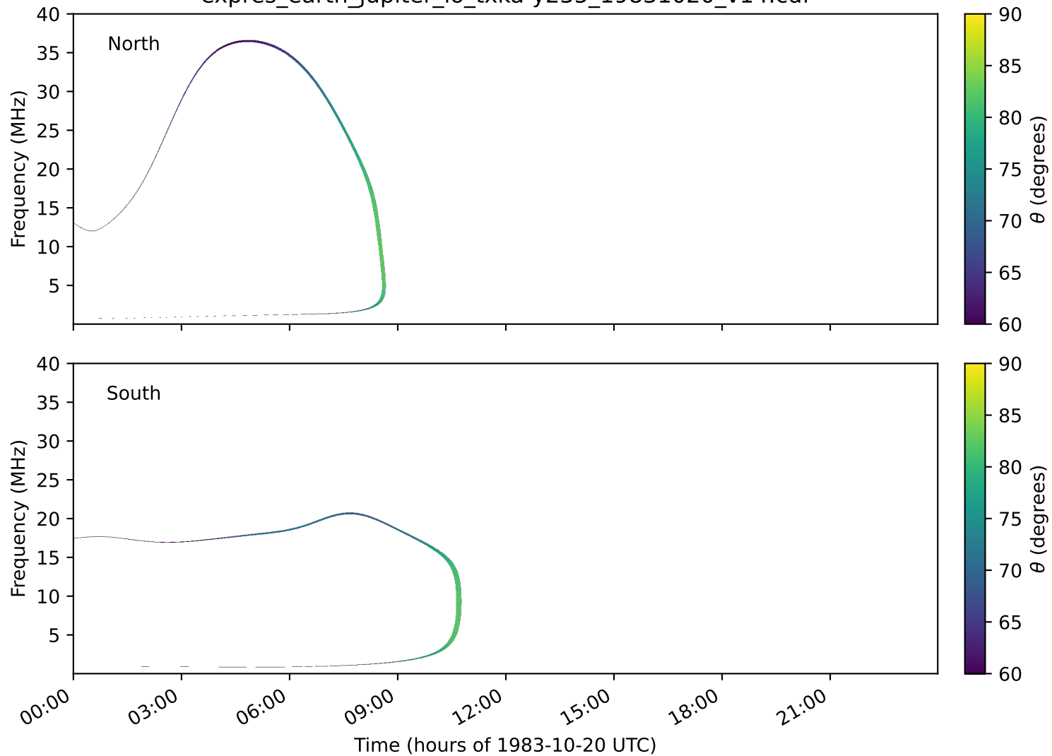
expres_earth_jupiter_io_txka-y235_19831020_v14.cdf
