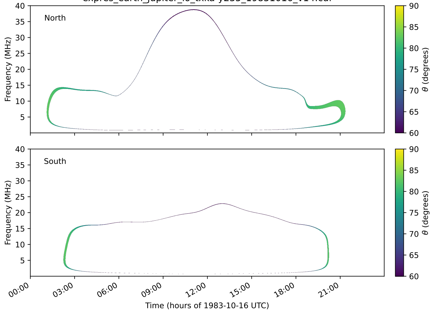
expres_earth_jupiter_io_txka-y235_19831016_v14.cdf
