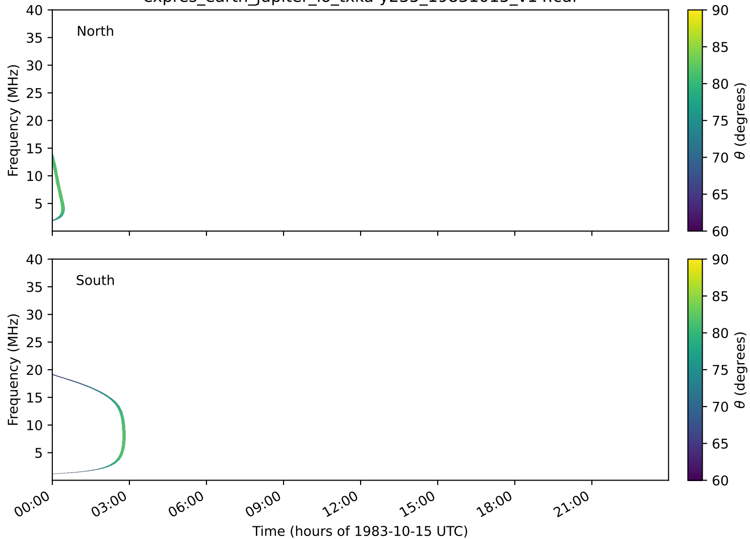
expres_earth_jupiter_io_txka-y235_19831015_v14.cdf
