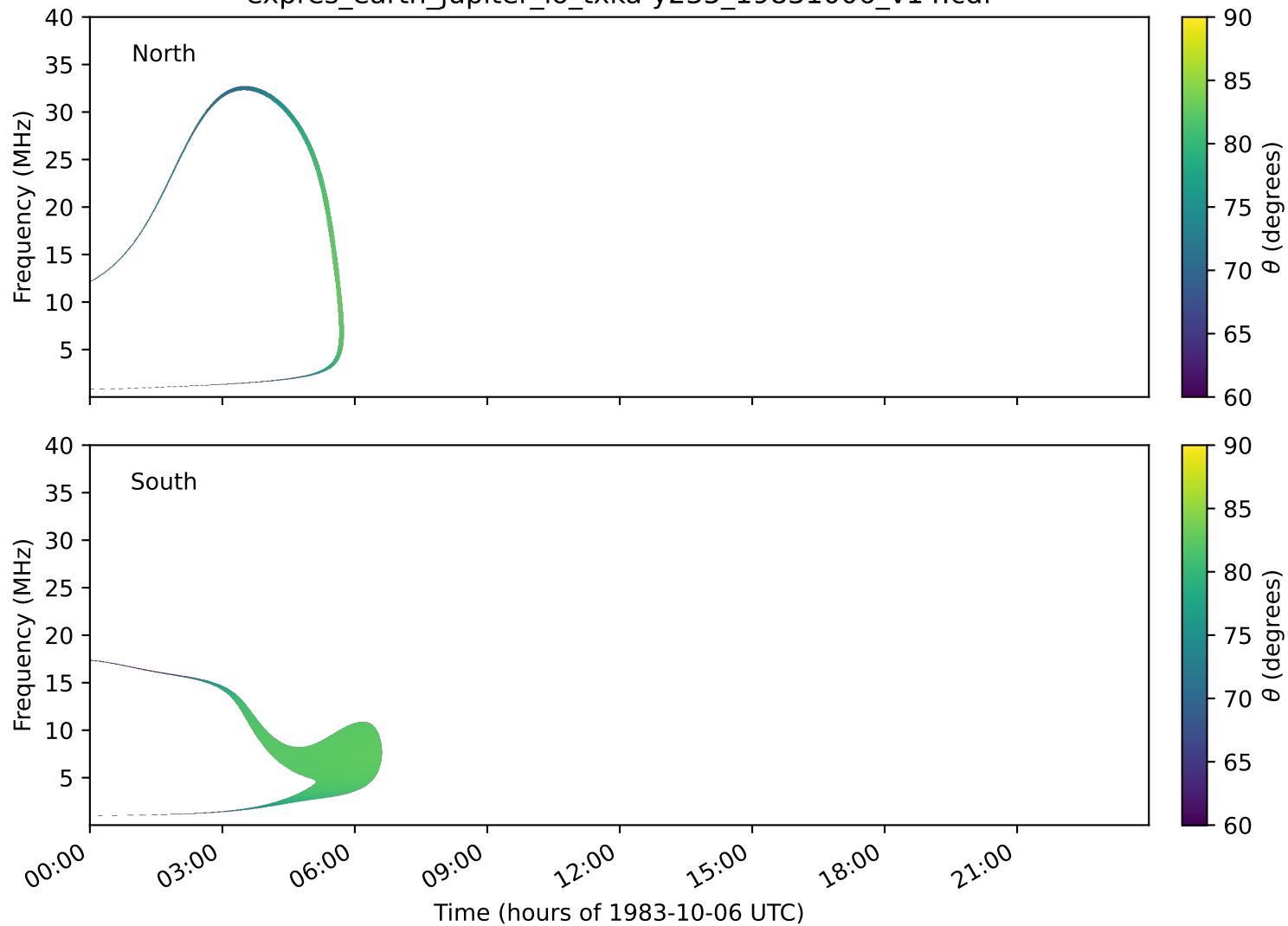
expres_earth_jupiter_io_txka-y235_19831006_v14.cdf
