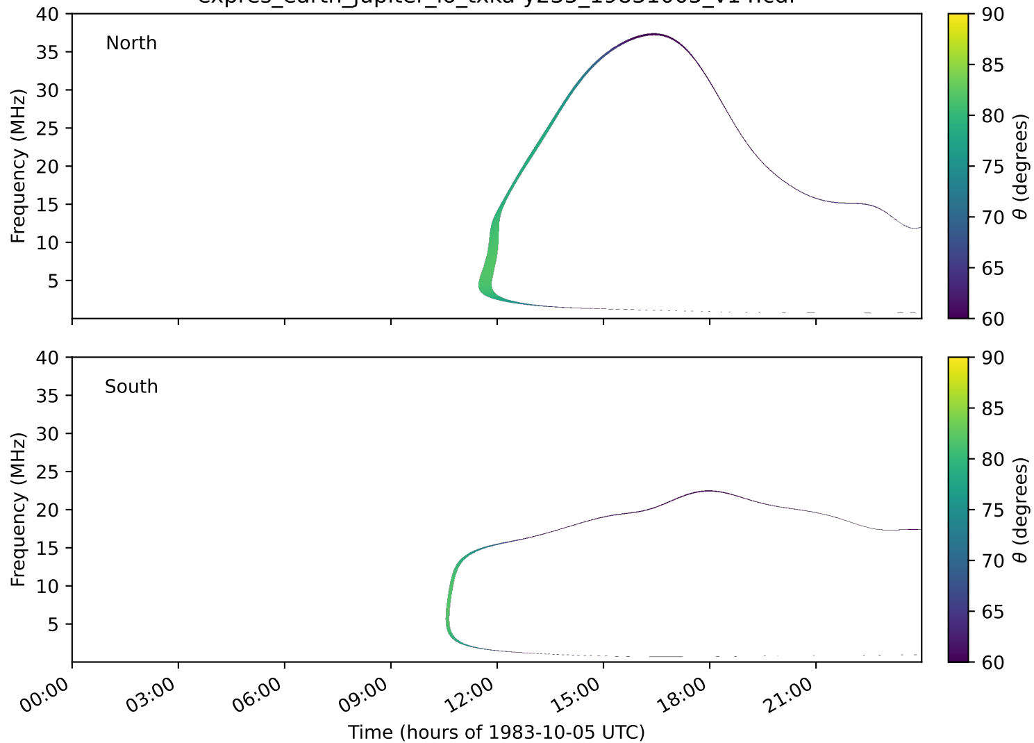
expres_earth_jupiter_io_txka-y235_19831005_v14.cdf
