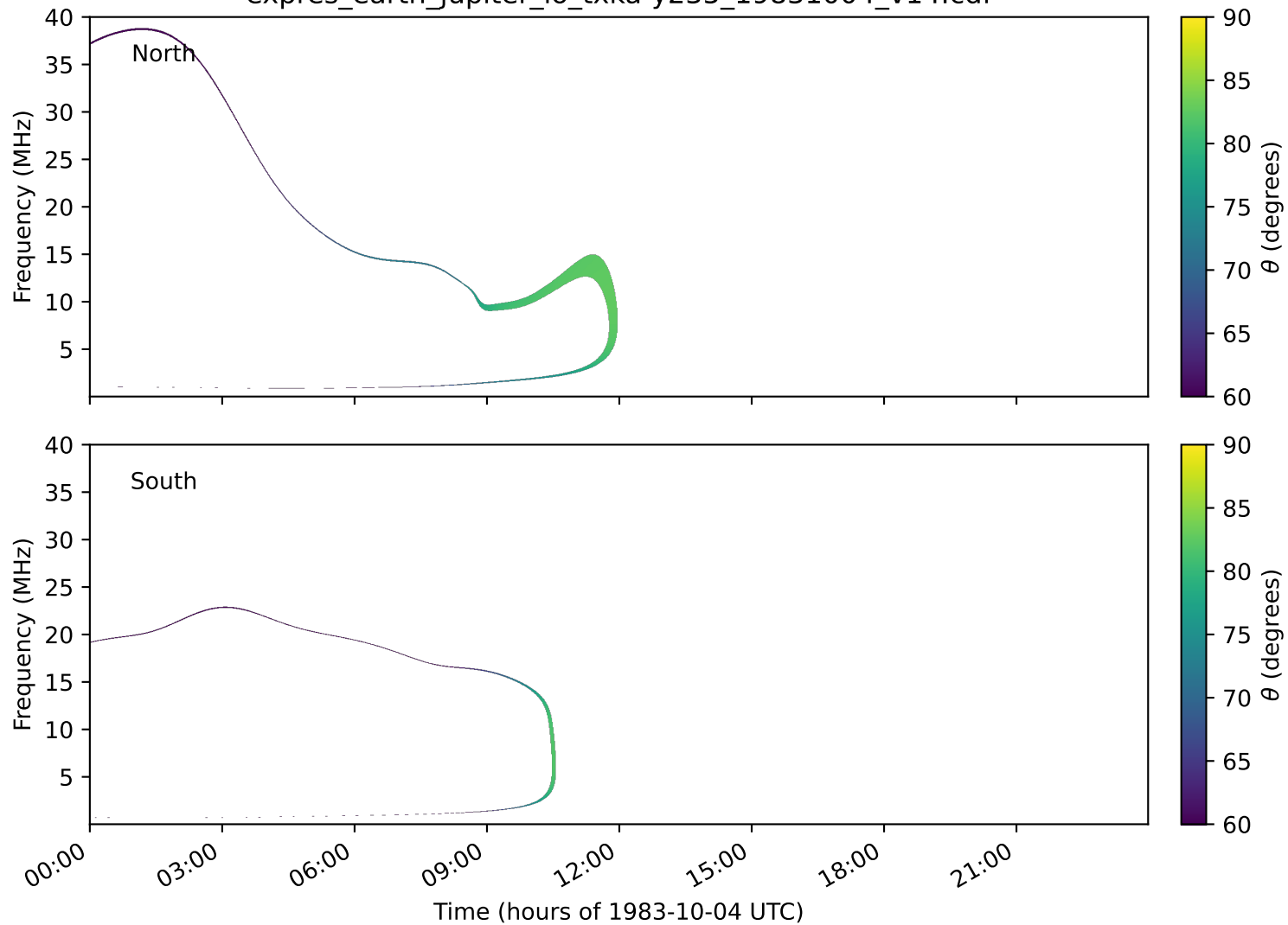
expres_earth_jupiter_io_txka-y235_19831004_v14.cdf
