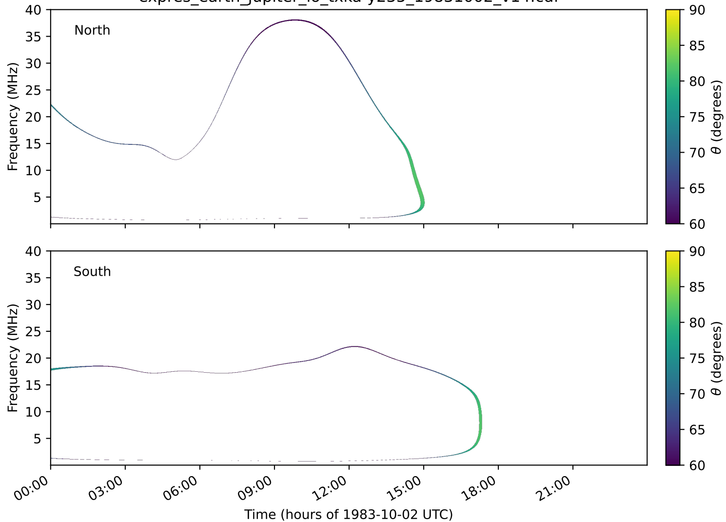
expres_earth_jupiter_io_txka-y235_19831002_v14.cdf
