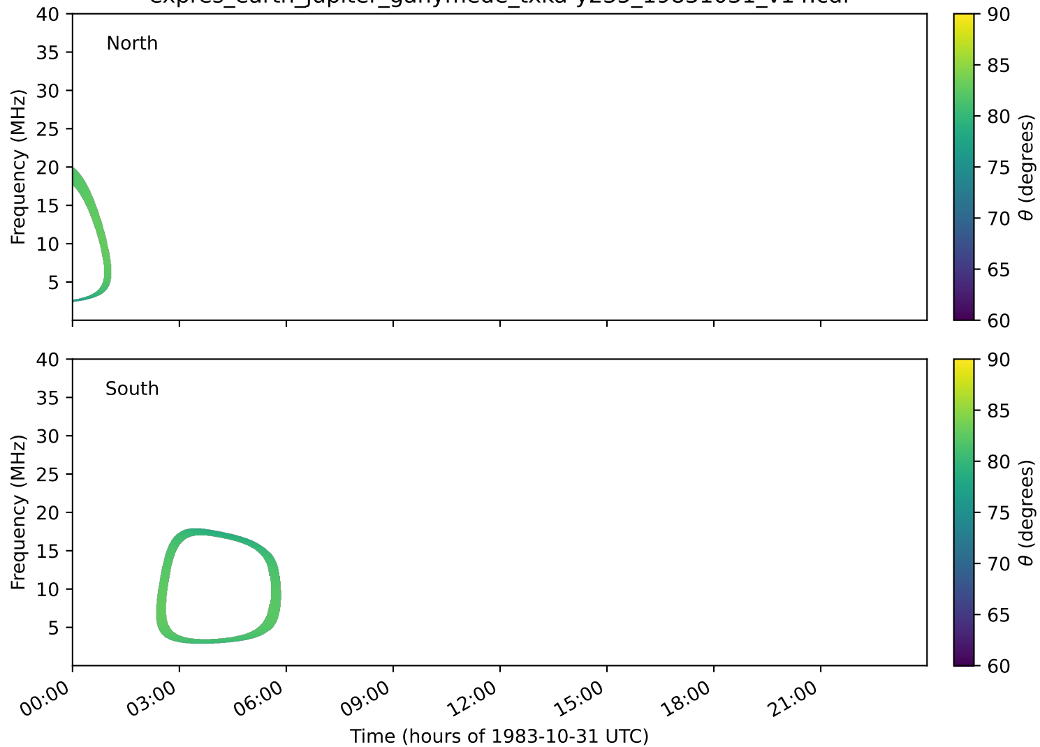
expres_earth_jupiter_ganymede_txka-y235_19831031_v14.cdf
