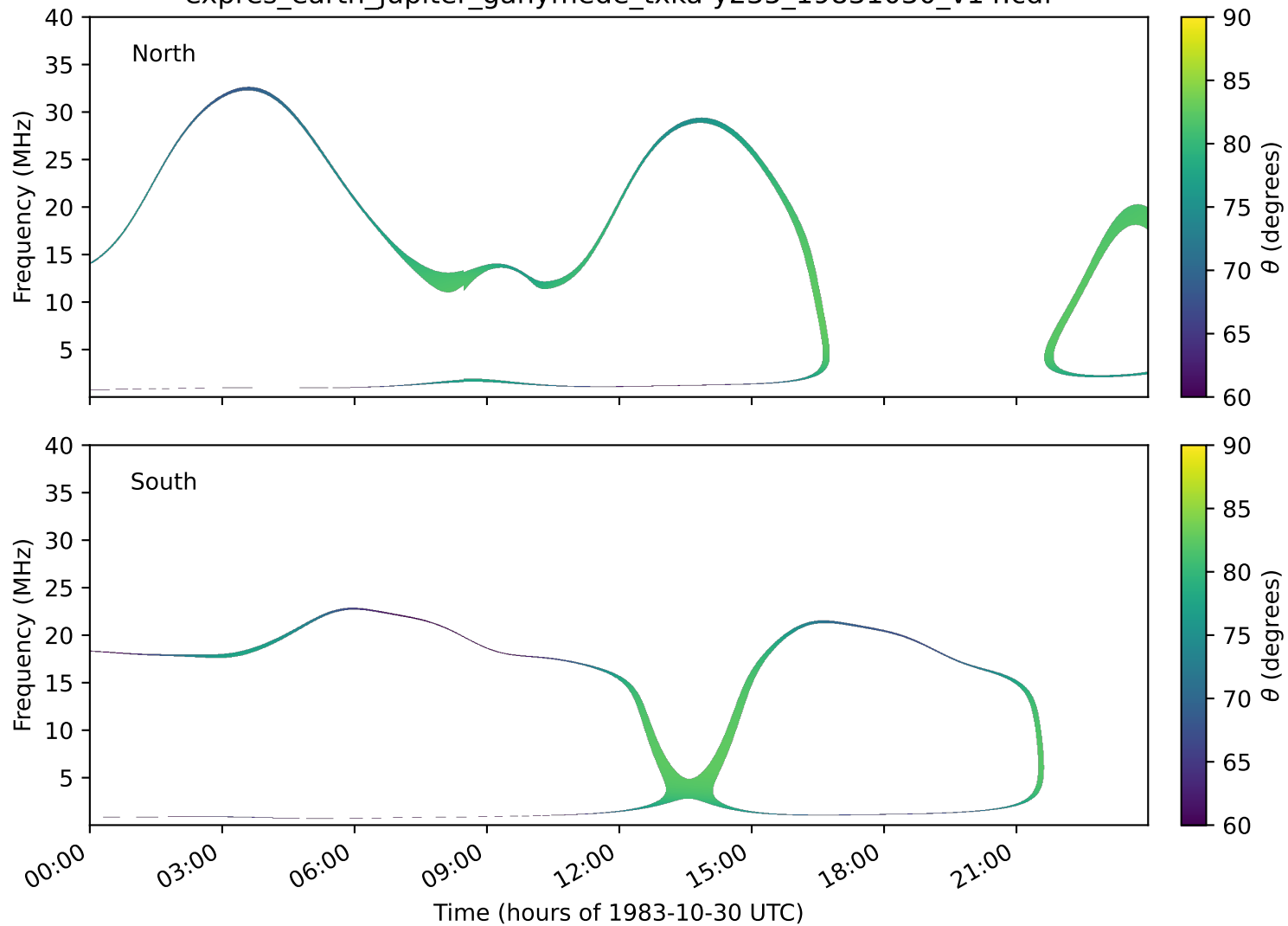
expres_earth_jupiter_ganymede_txka-y235_19831030_v14.cdf
