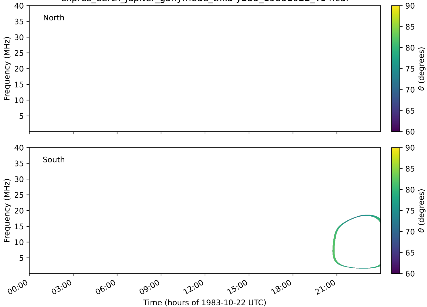
expres_earth_jupiter_ganymede_txka-y235_19831022_v14.cdf
