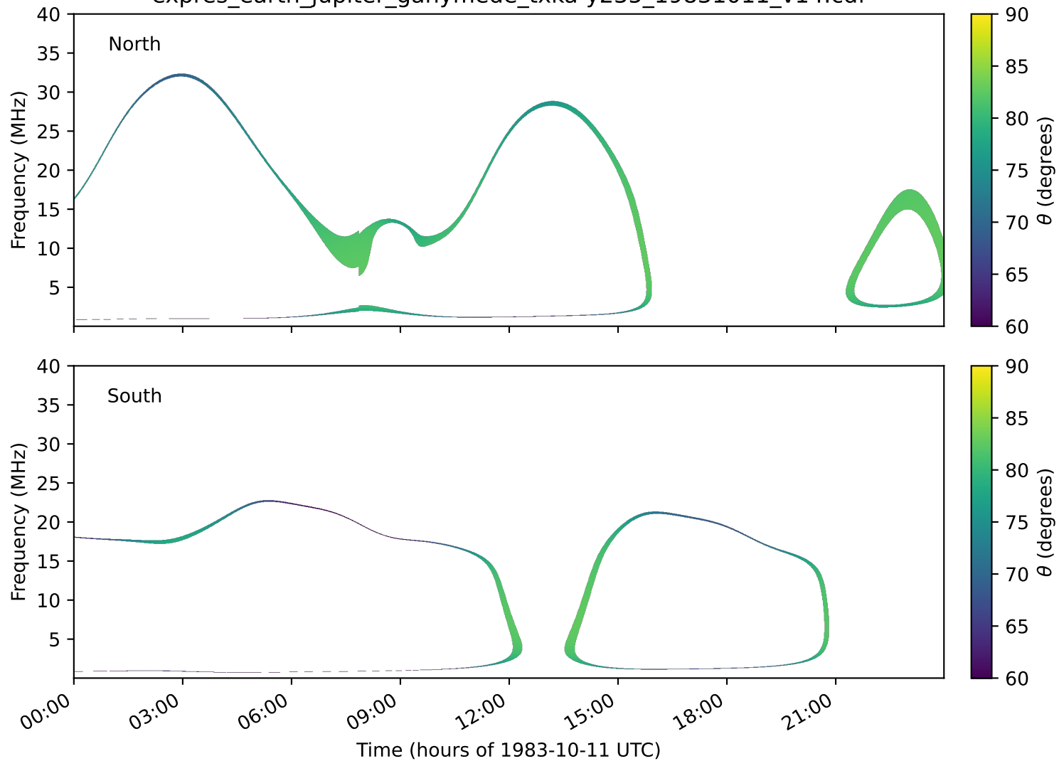
expres_earth_jupiter_ganymede_txka-y235_19831011_v14.cdf
