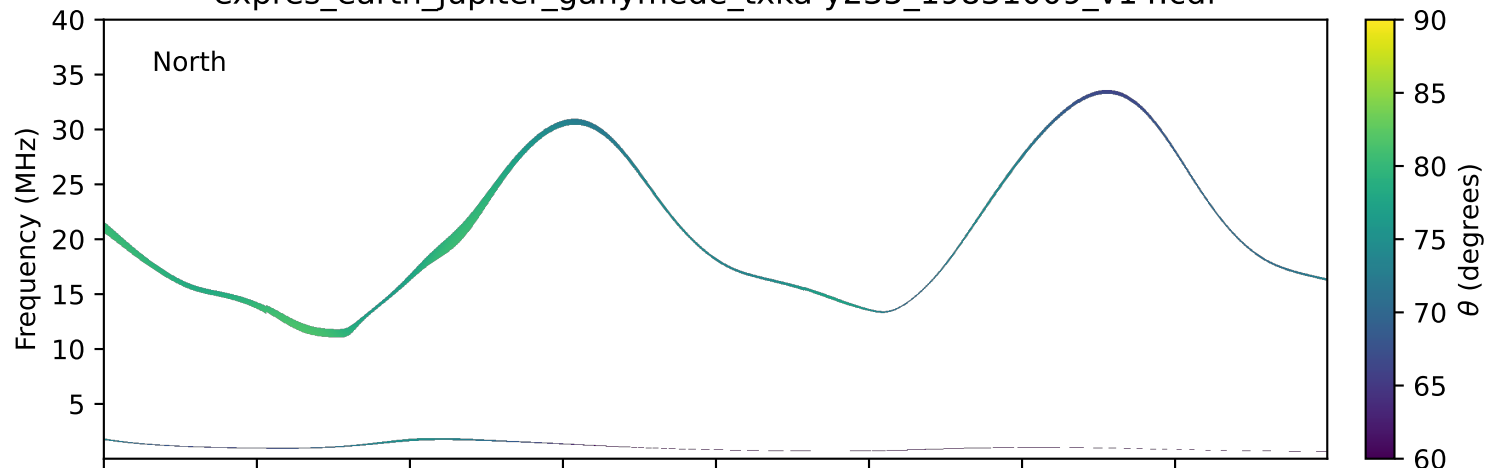
expres_earth_jupiter_ganymede_txka-y235_19831009_v14.cdf
