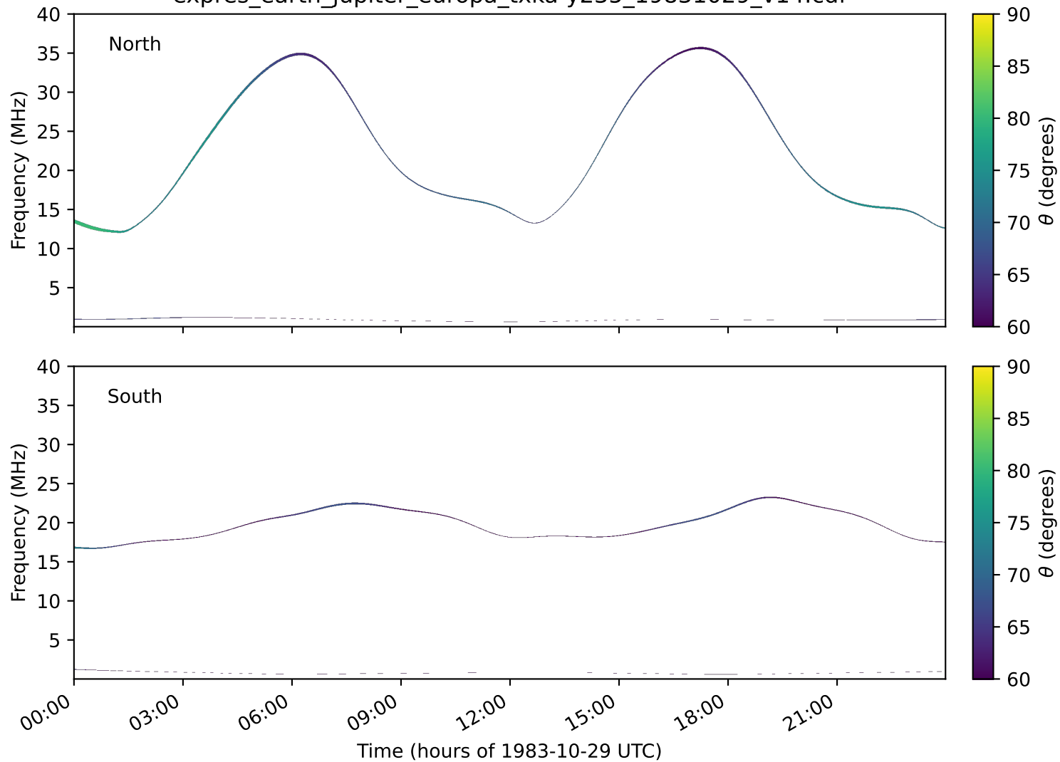
expres_earth_jupiter_europa_txka-y235_19831029_v14.cdf
