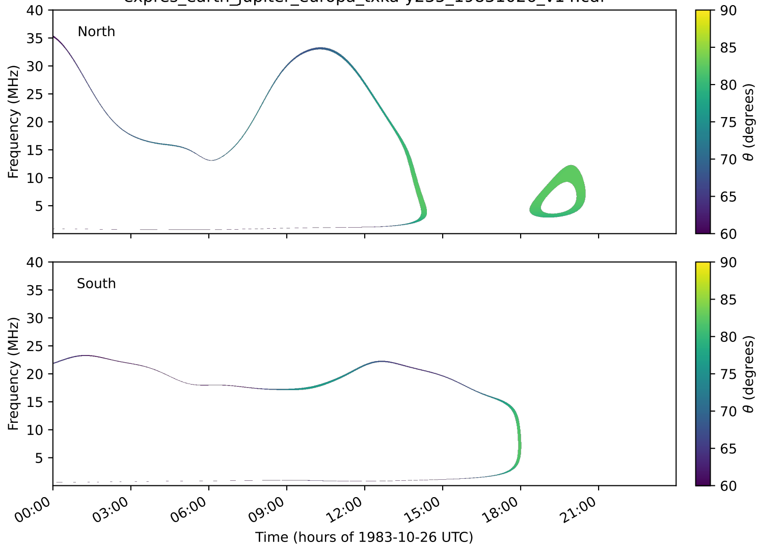
expres_earth_jupiter_europa_txka-y235_19831026_v14.cdf
