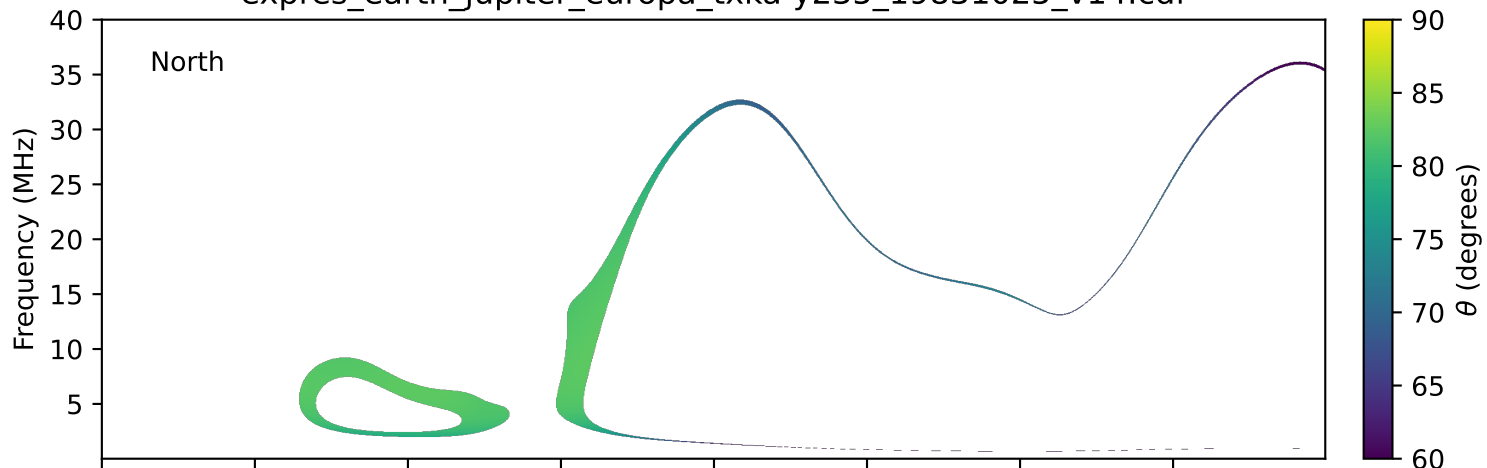
expres_earth_jupiter_europa_txka-y235_19831025_v14.cdf
