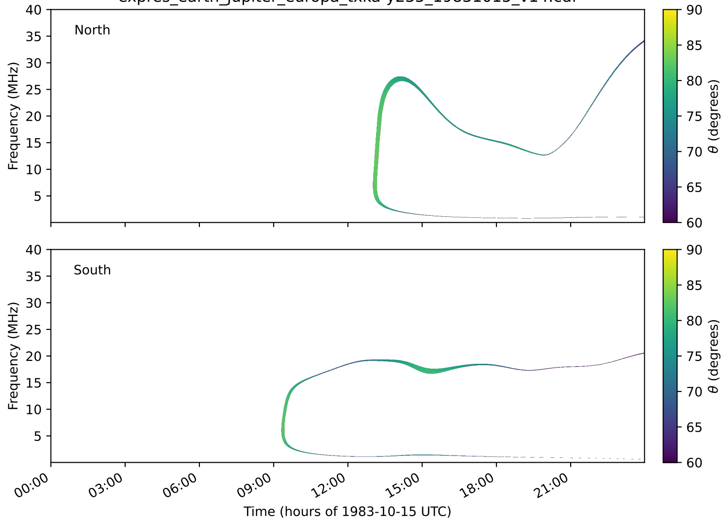
expres_earth_jupiter_europa_txka-y235_19831015_v14.cdf
