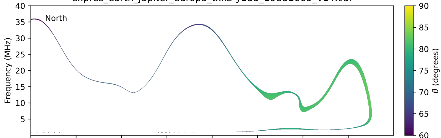
expres_earth_jupiter_europa_txka-y235_19831009_v14.cdf
