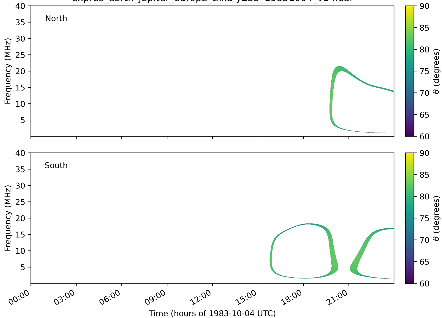
expres_earth_jupiter_europa_txka-y235_19831004_v14.cdf
