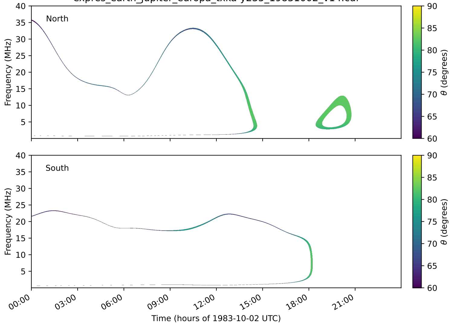
expres_earth_jupiter_europa_txka-y235_19831002_v14.cdf
