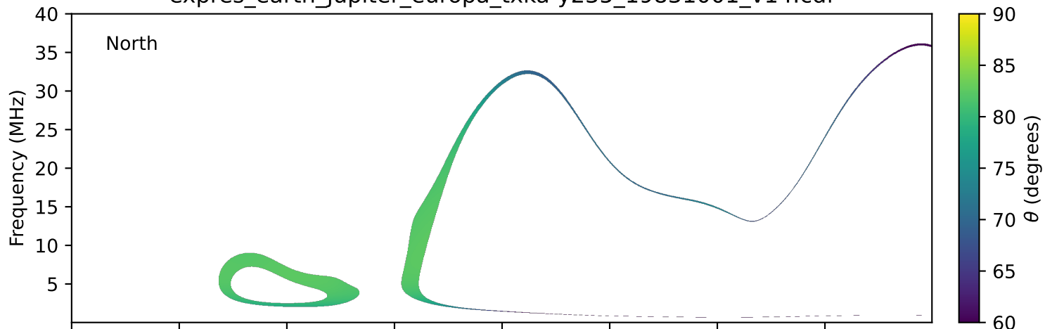
expres_earth_jupiter_europa_txka-y235_19831001_v14.cdf
