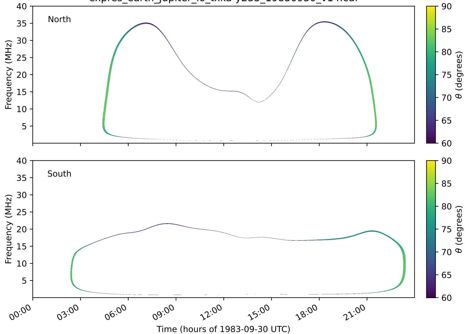
expres_earth_jupiter_io_txka-y235_19830930_v14.cdf
