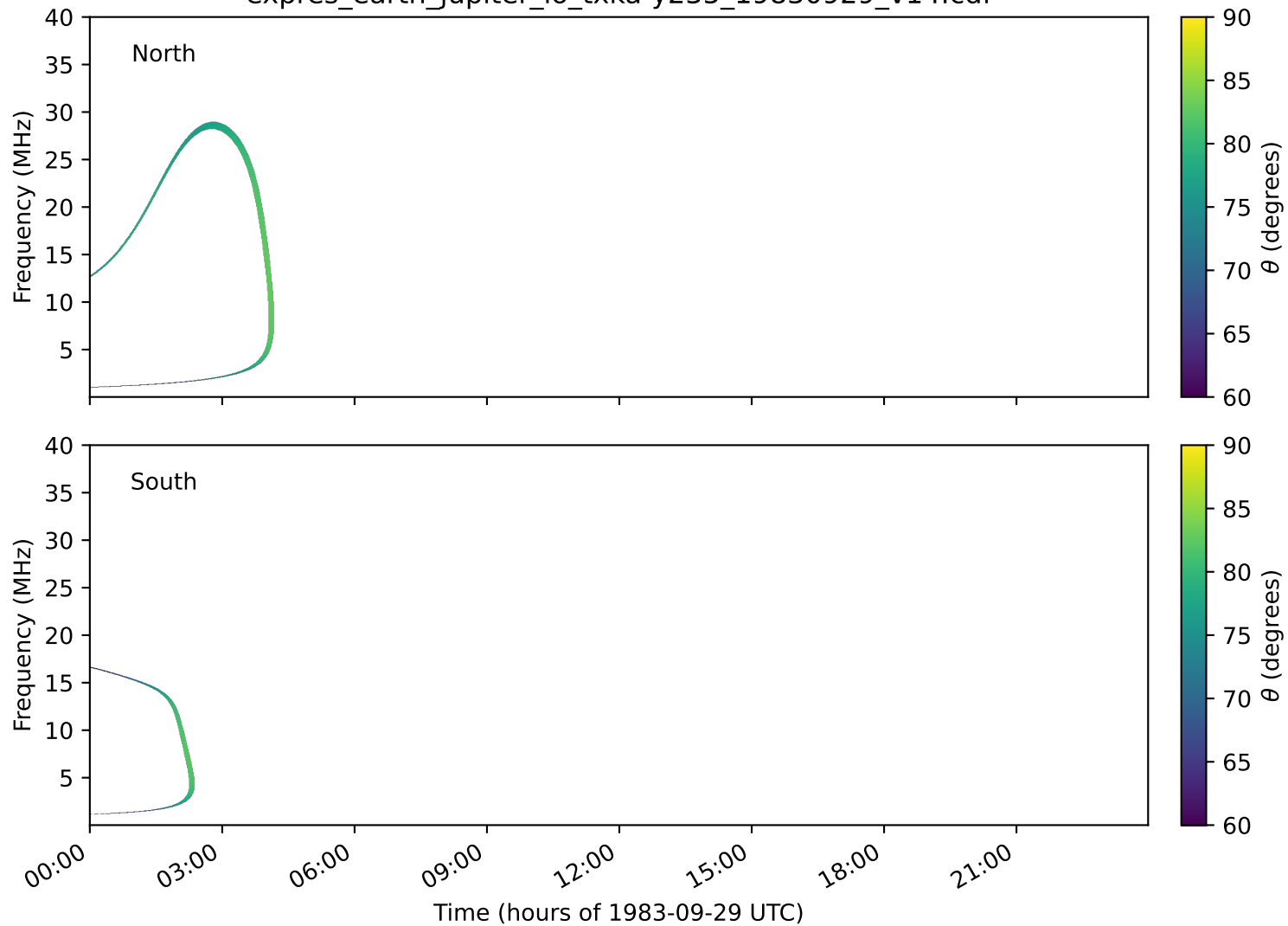
expres_earth_jupiter_io_txka-y235_19830929_v14.cdf
