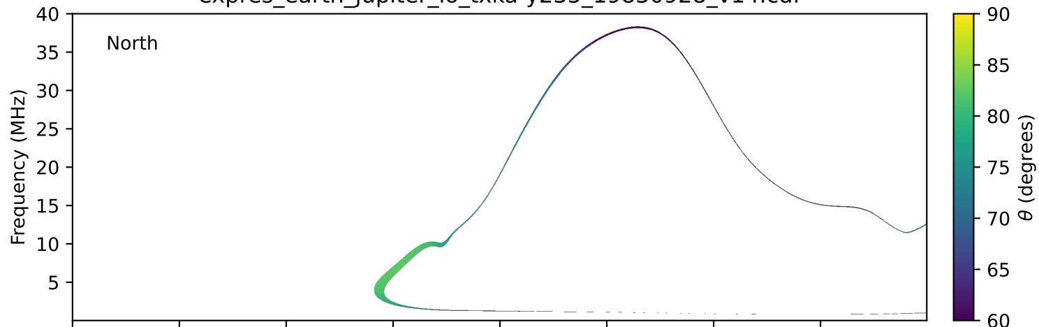
expres_earth_jupiter_io_txka-y235_19830928_v14.cdf
