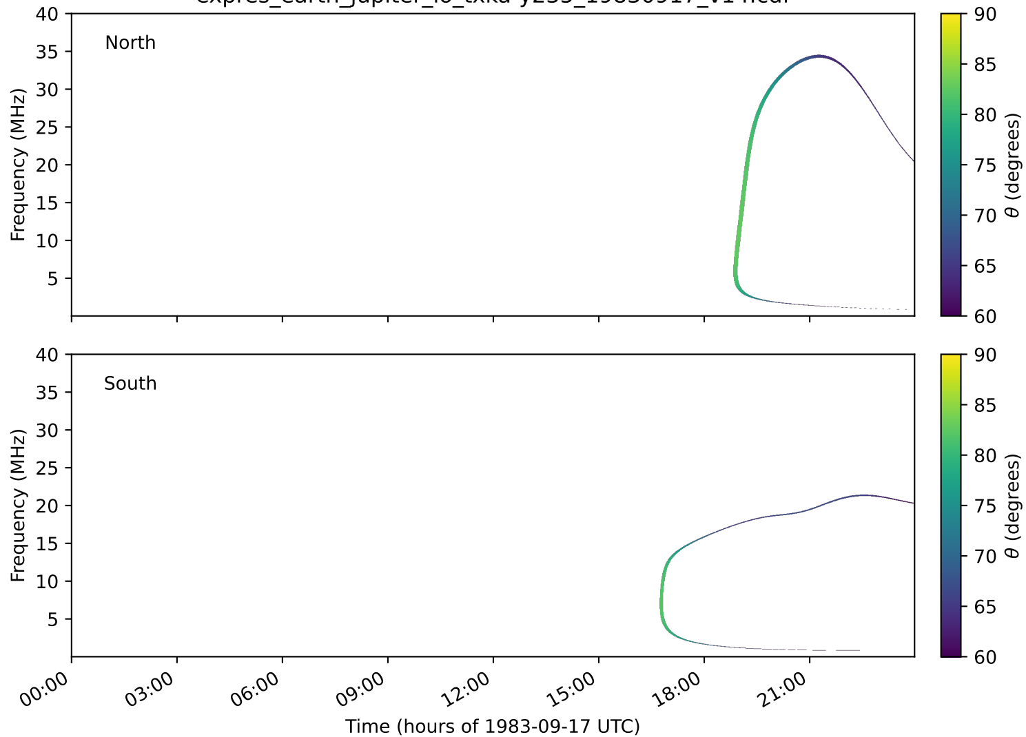
expres_earth_jupiter_io_txka-y235_19830917_v14.cdf
