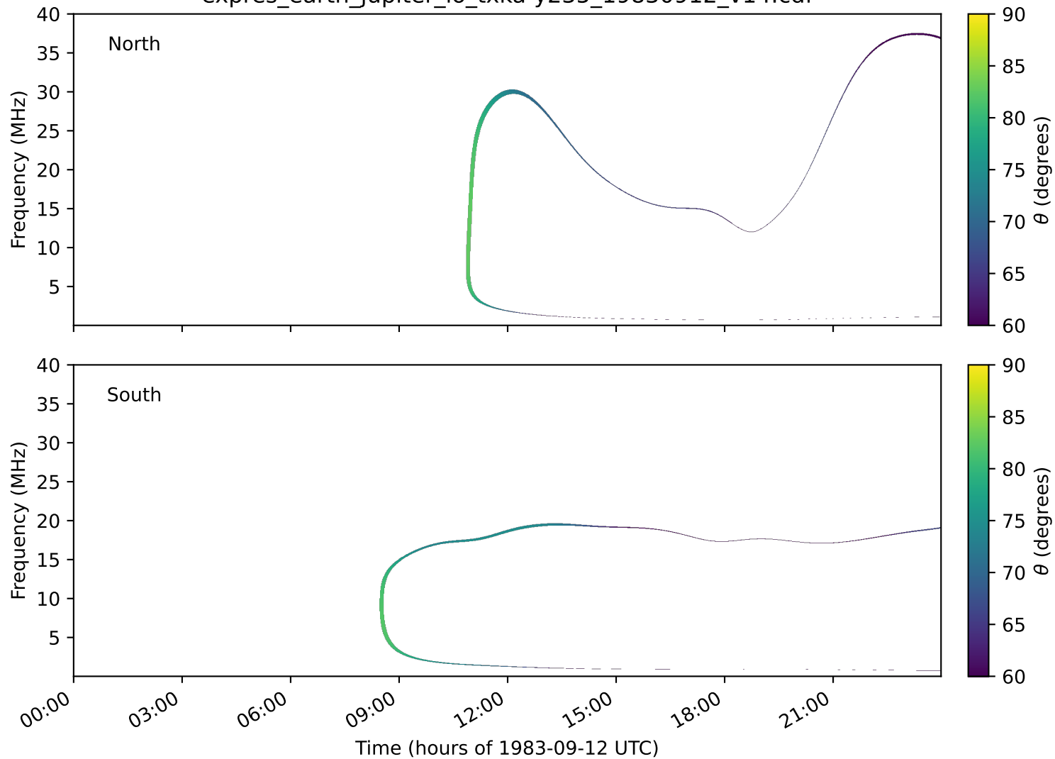
expres_earth_jupiter_io_txka-y235_19830912_v14.cdf
