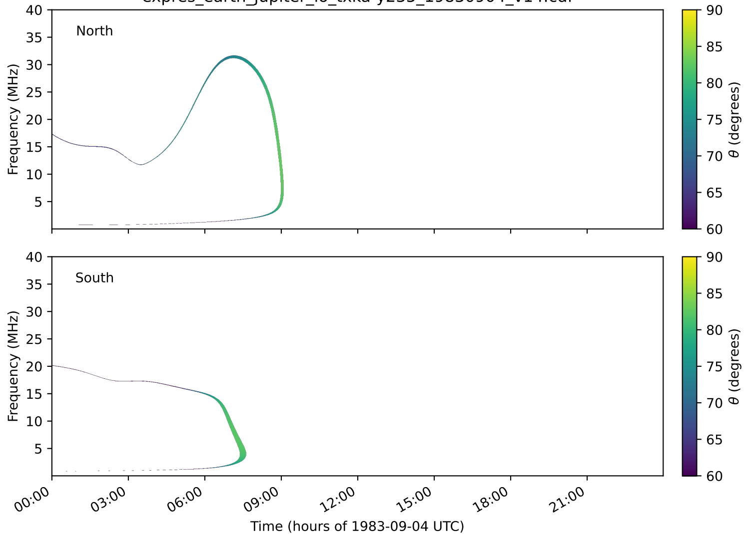
expres_earth_jupiter_io_txka-y235_19830904_v14.cdf
