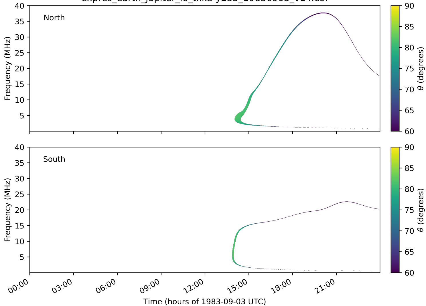
expres_earth_jupiter_io_txka-y235_19830903_v14.cdf
