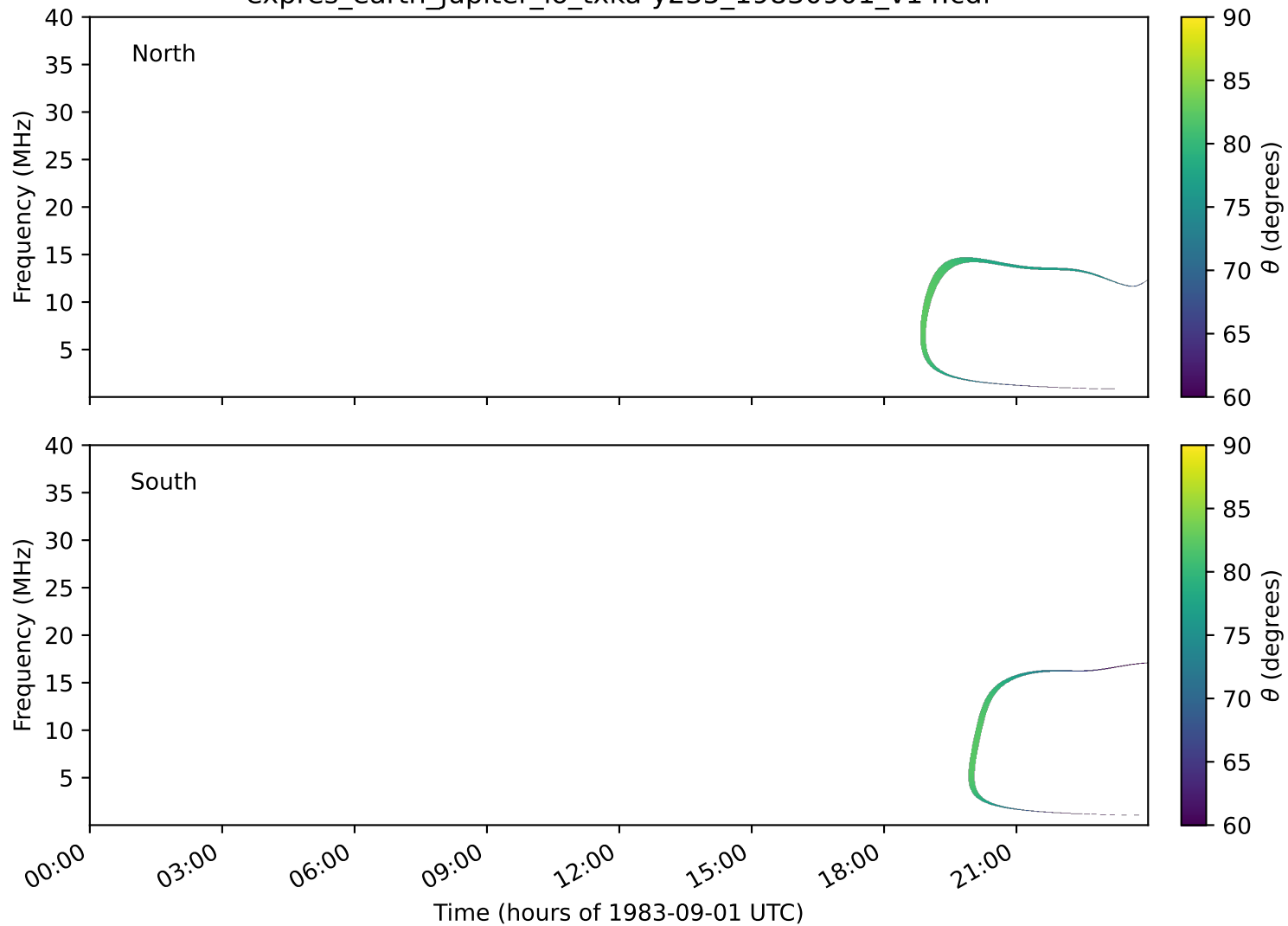
expres_earth_jupiter_io_txka-y235_19830901_v14.cdf
