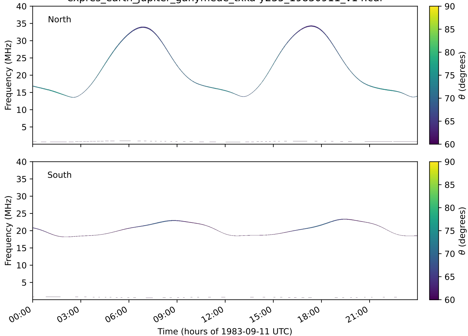
expres_earth_jupiter_ganymede_txka-y235_19830911_v14.cdf
