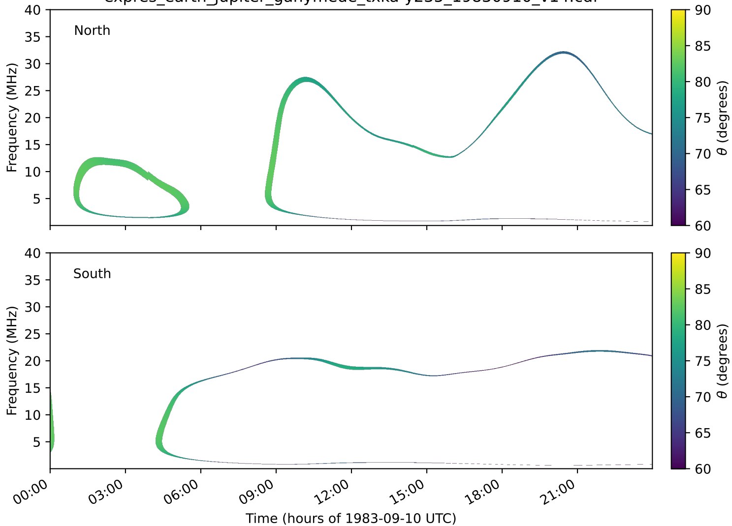
expres_earth_jupiter_ganymede_txka-y235_19830910_v14.cdf
